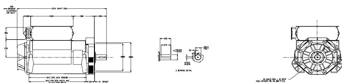
P80 W/X CORES
